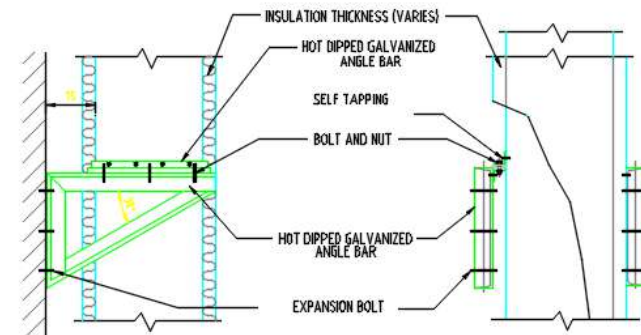
WALL BRACKET FOR INSULATED DUCT
