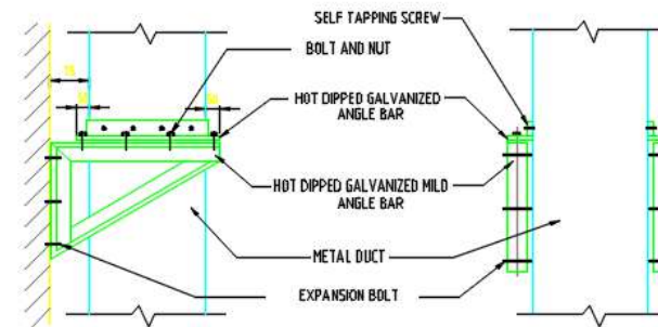
WALL BRACKET FOR NON-INSULATED DUCT
