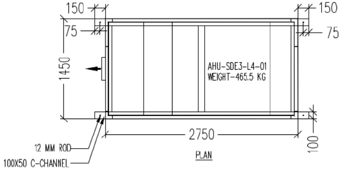
INSTALLATION DETAIL FOR HANGING AHU
